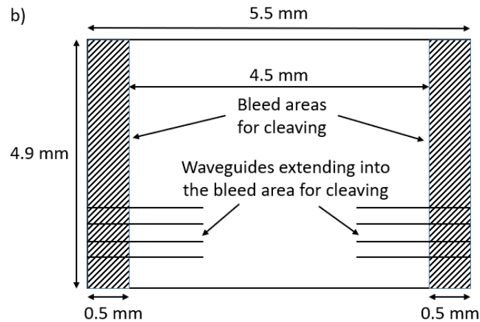
Figure 1 – User cell design area layout for a) 11.47 \times 4.9 \text{ mm}^2 , and b) 5.5 \times 4.9 \text{ mm}^2 .
