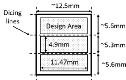
Figure 1 – Physical die dimensions.
