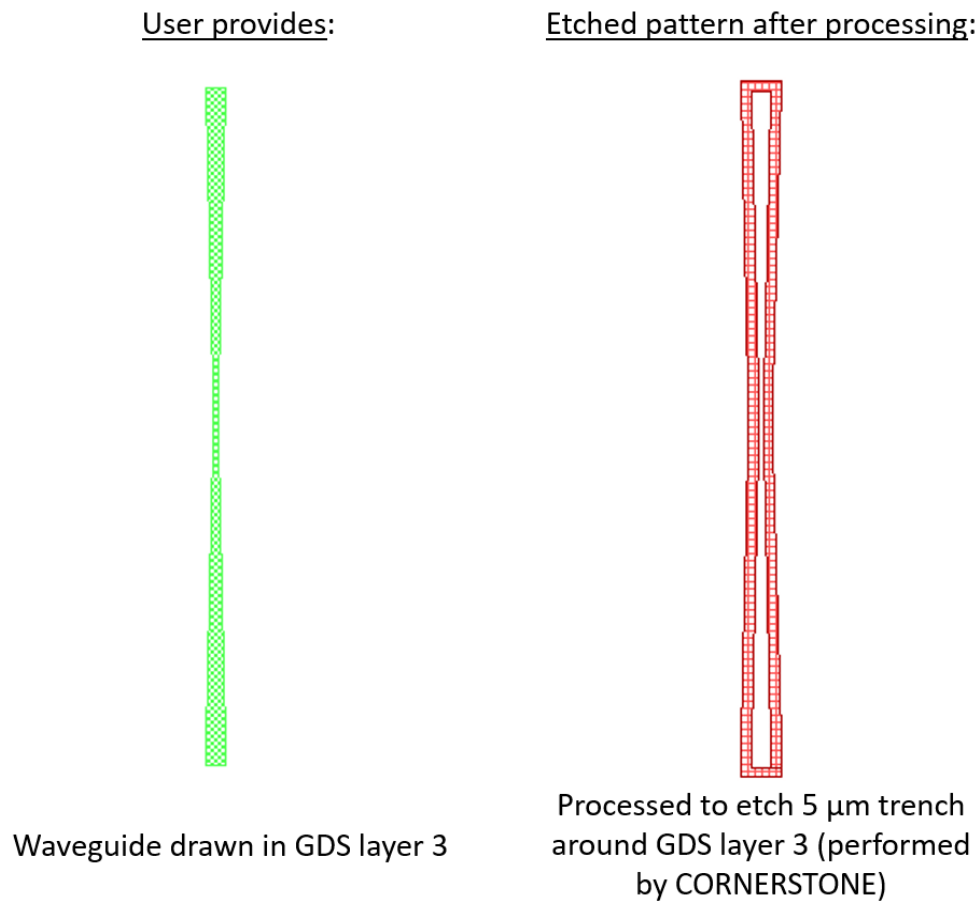
Figure 2 – Description of GDS Layer 3 processing.
