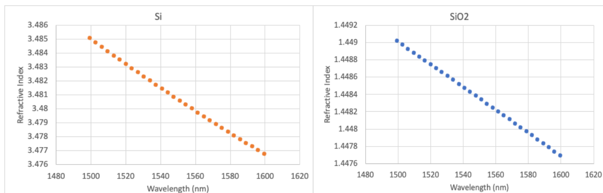
Figure 5 – Refractive indices of Silicon(left) and \text{SiO}_2 (right).
