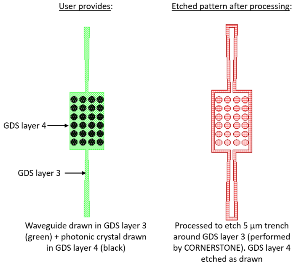
Figure 3 – Example photonic crystal structure using GDS Layers 3 & 4.
